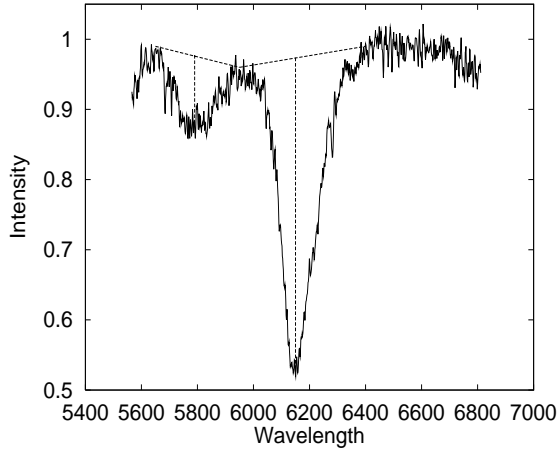
Fig. 3. Graphical representation of the method of measuring line depth ratio of the two Si II lines.
